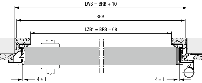
Horizontal view
