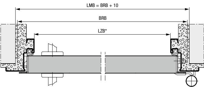
Horizontal view
