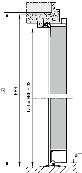
Vertical view
