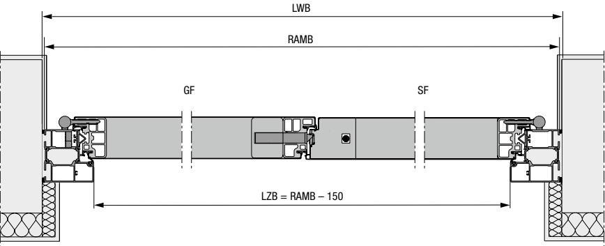
Horizontal view
