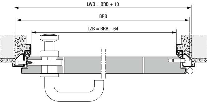
Frame variants
