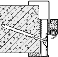
Diagonal fixing With counter frame Vario B53 as a double-shell profile frame (Gas concrete)
