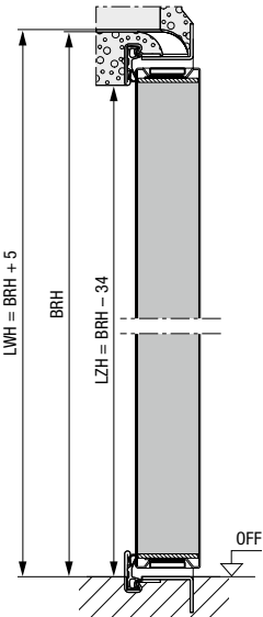
Vertical view
