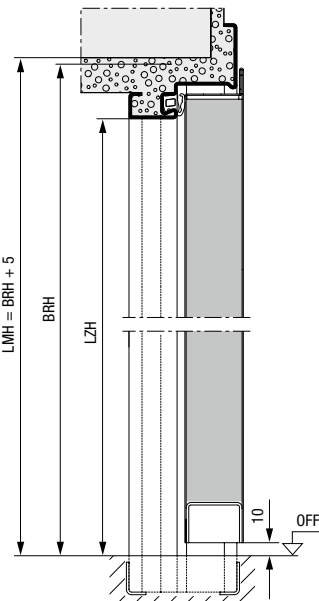
Vertical view
